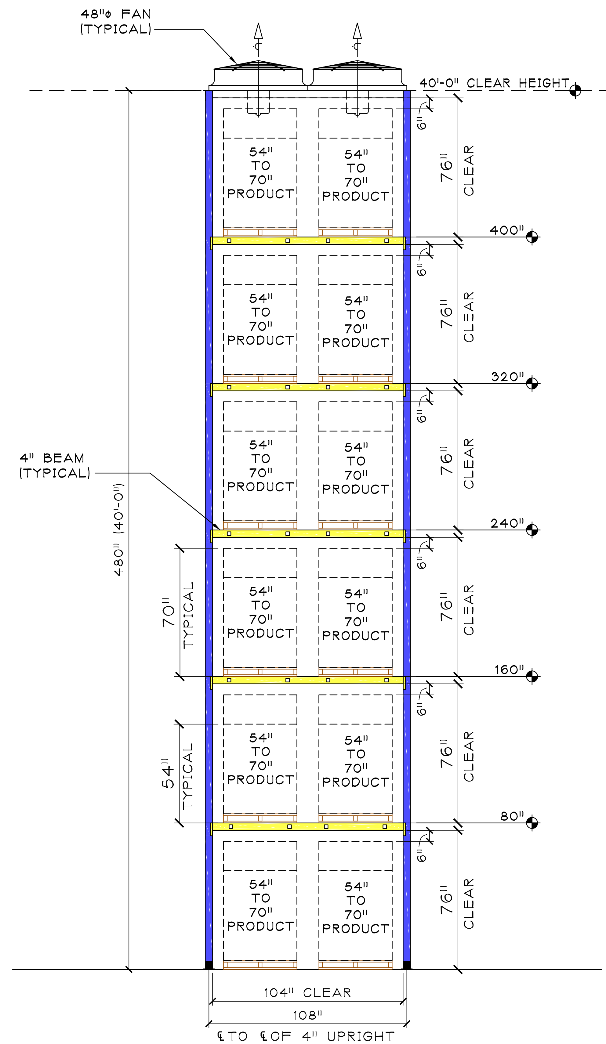
A FRONT VIEW STOCK QUICKFREEZE BAY 6-HIGH PALLETS
